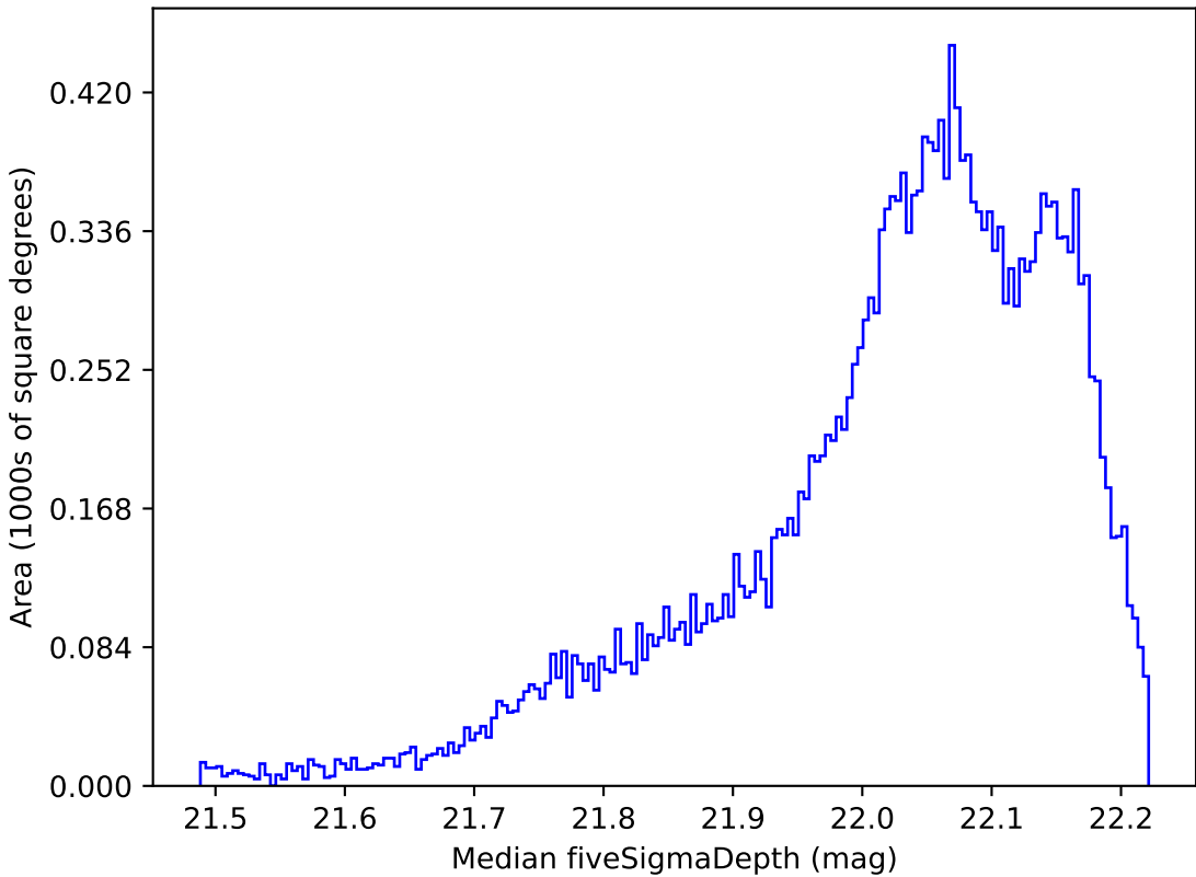
noroll_mjdp60_v3.4_10yrs All sky y band: Median fiveSigmaDepth
