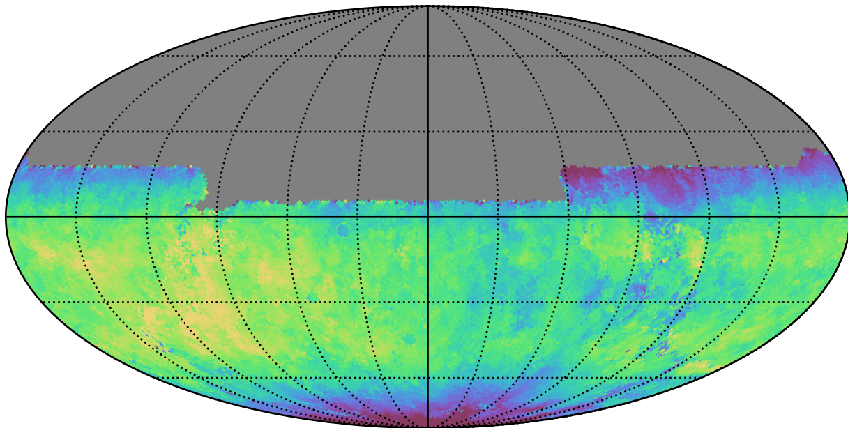
noroll_mjdp60_v3.4_10yrs All sky u band: Median fiveSigmaDepth
