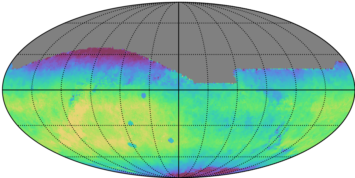
noroll_mjdp60_v3.4_10yrs All sky r band: Median fiveSigmaDepth
