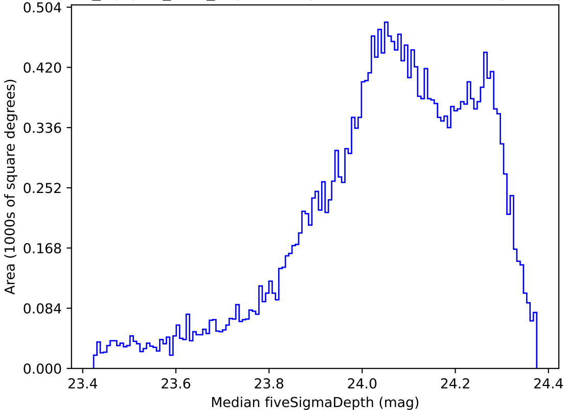
noroll_mjdp60_v3.4_10yrs All sky r band: Median fiveSigmaDepth
