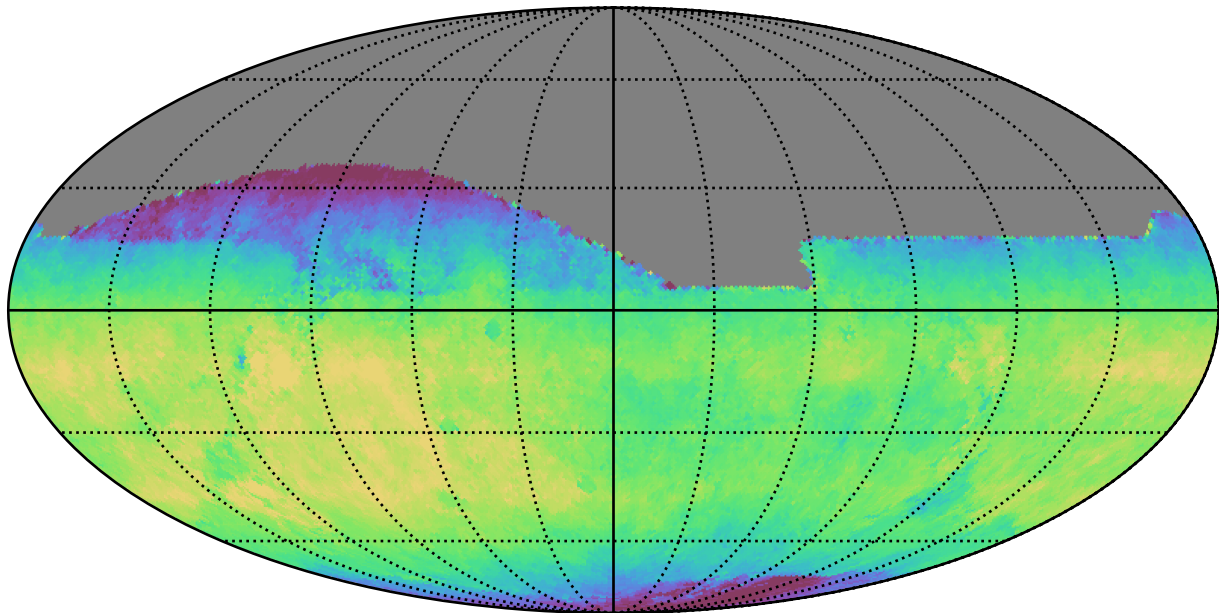
noroll_mjdp60_v3.4_10yrs All sky i band: Median fiveSigmaDepth
