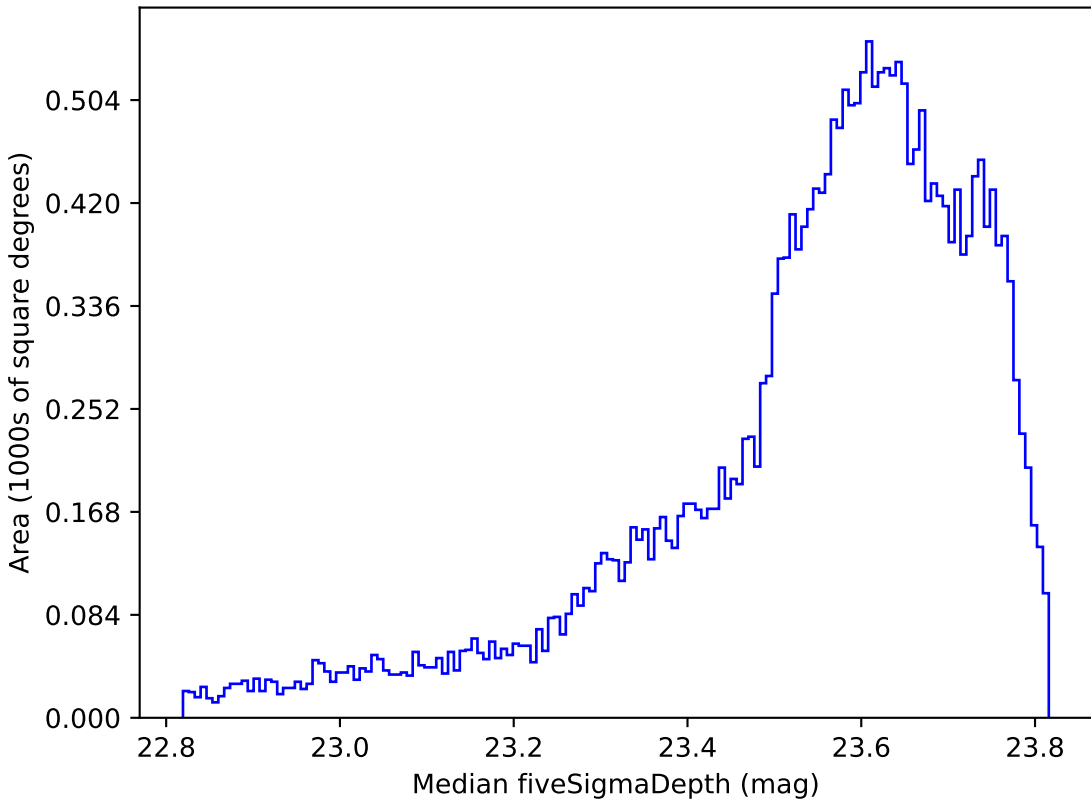
noroll_mjdp60_v3.4_10yrs All sky i band: Median fiveSigmaDepth
