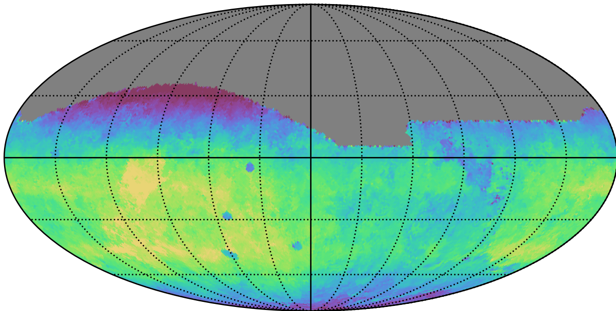
noroll_mjdp60_v3.4_10yrs All sky g band: Median fiveSigmaDepth
