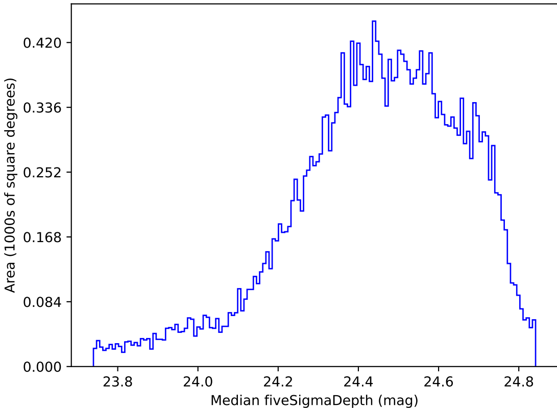
noroll_mjdp60_v3.4_10yrs All sky g band: Median fiveSigmaDepth
