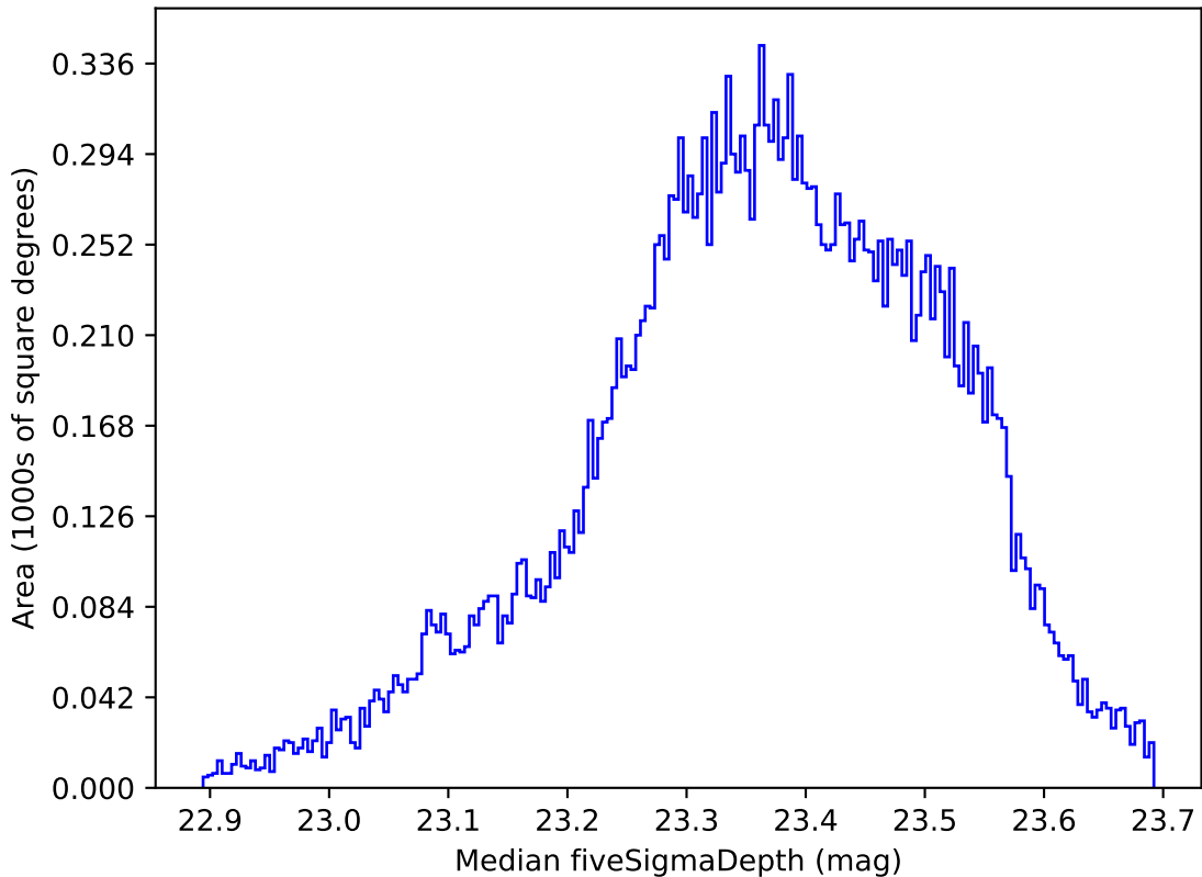
noroll_mjdp60_v3.4_10yrs All sky all bands: Median fiveSigmaDepth
