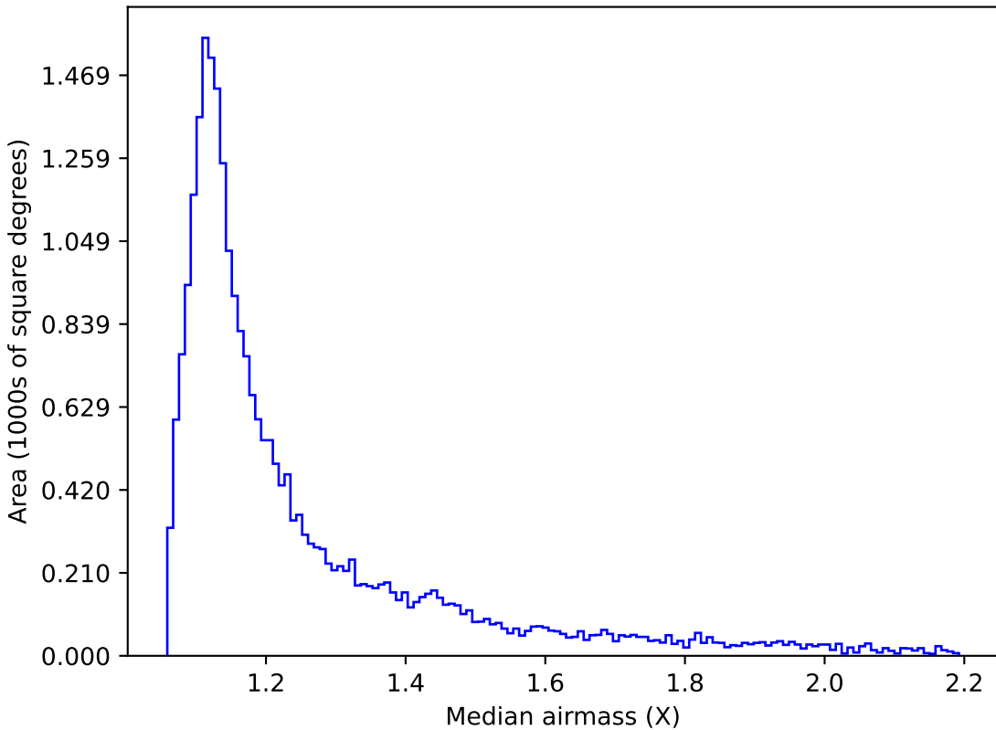
noroll_mjdp60_v3.4_10yrs Yr 1 z band: Median airmass
