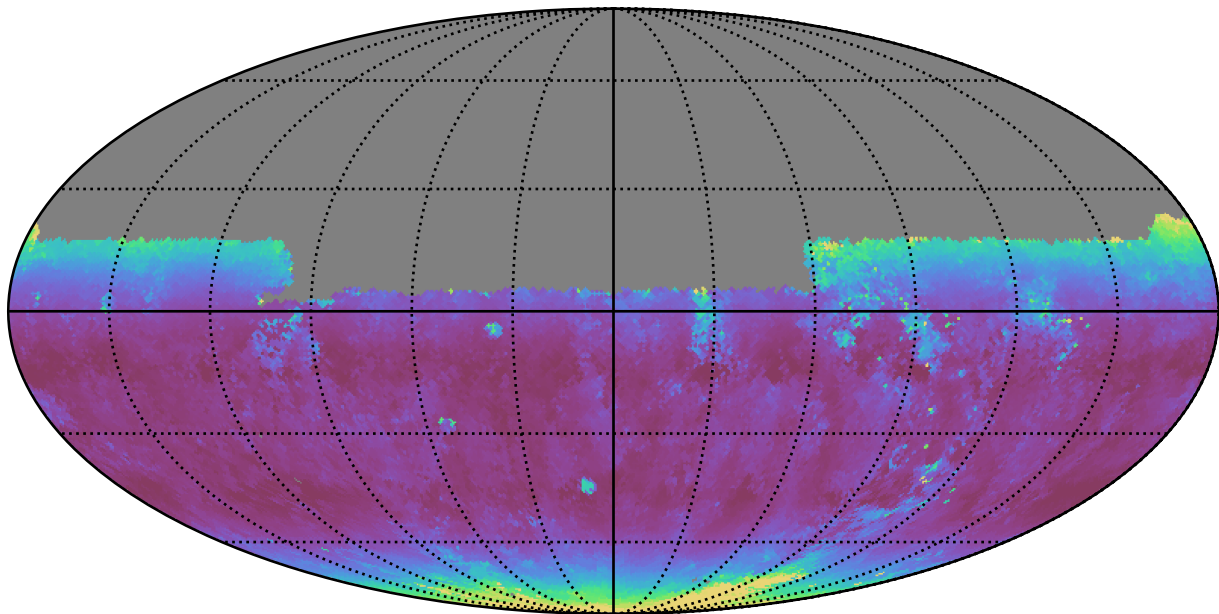
noroll_mjdp60_v3.4_10yrs Yr 1 y band: Median airmass
