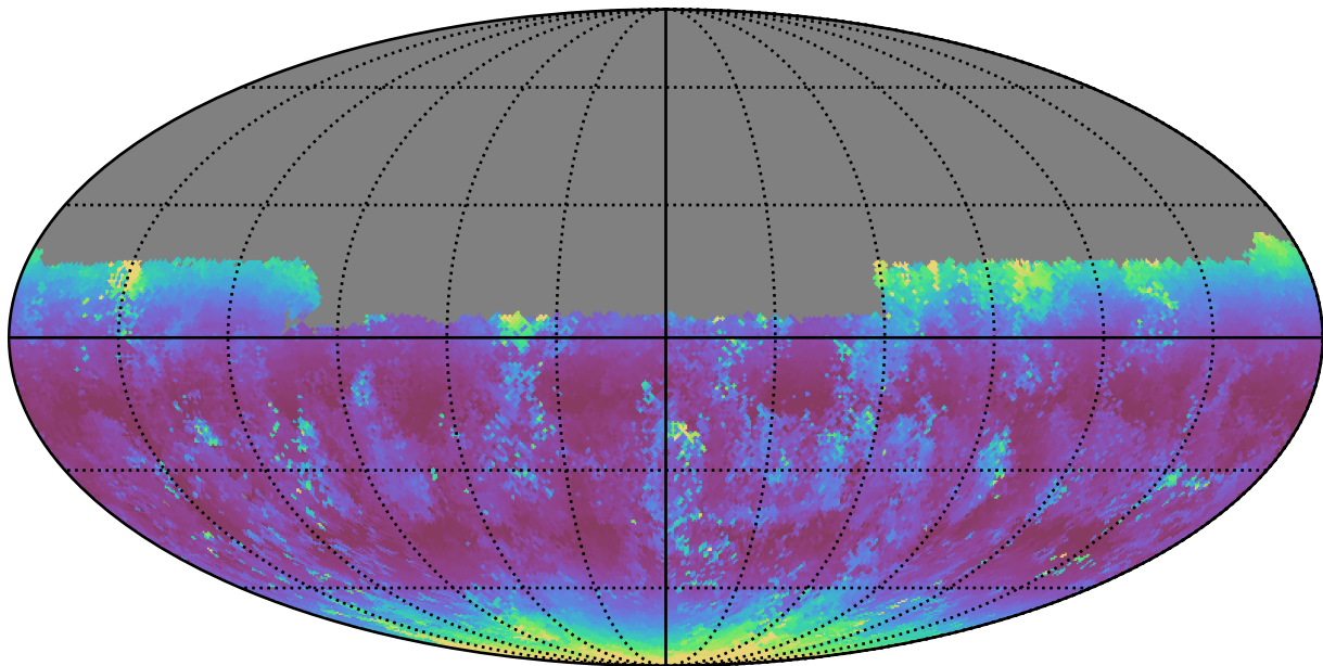
noroll_mjdp60_v3.4_10yrs Yr 1 u band: Median airmass
