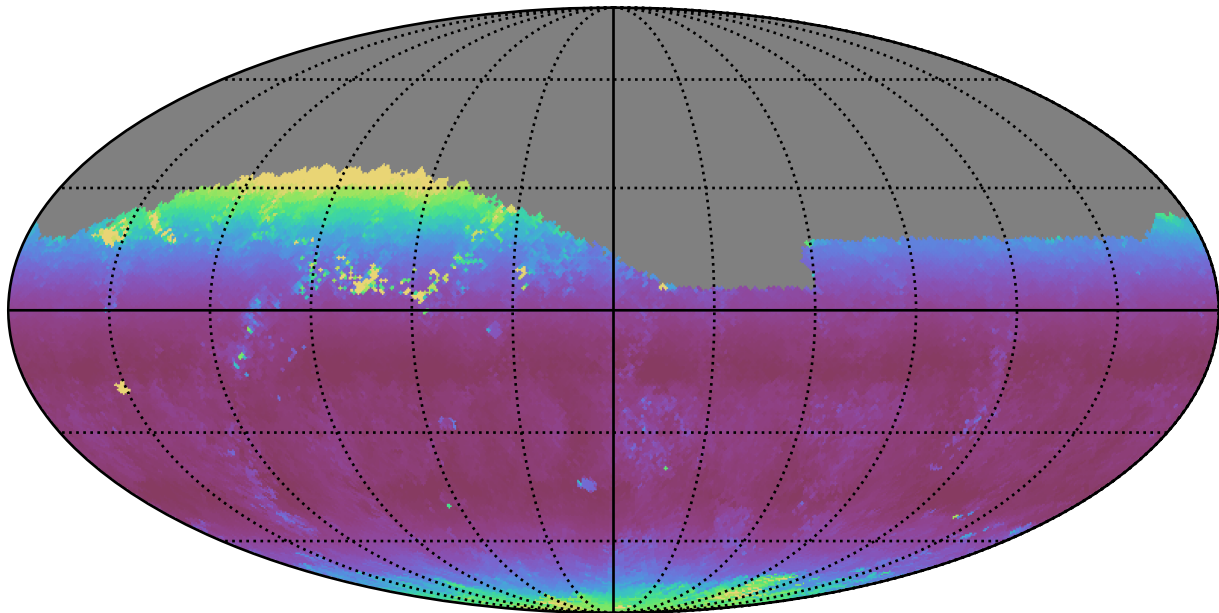
noroll_mjdp60_v3.4_10yrs Yr 1 i band: Median airmass
