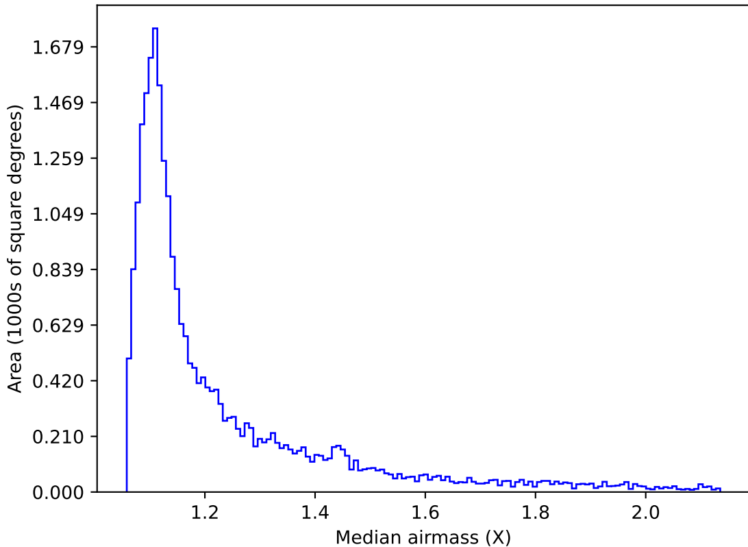
noroll_mjdp60_v3.4_10yrs Yr 1 i band: Median airmass
