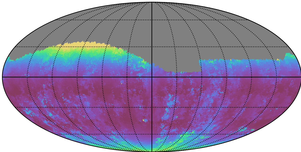
noroll_mjdp60_v3.4_10yrs Yr 1 g band: Median airmass
