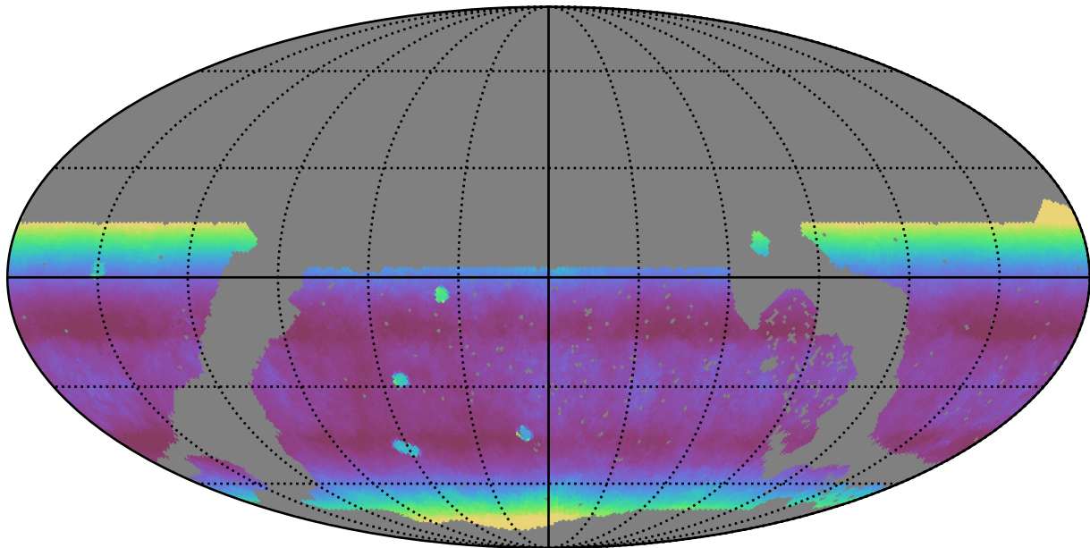
noroll_mjdp60_v3.4_10yrs WFD z band: Median airmass
