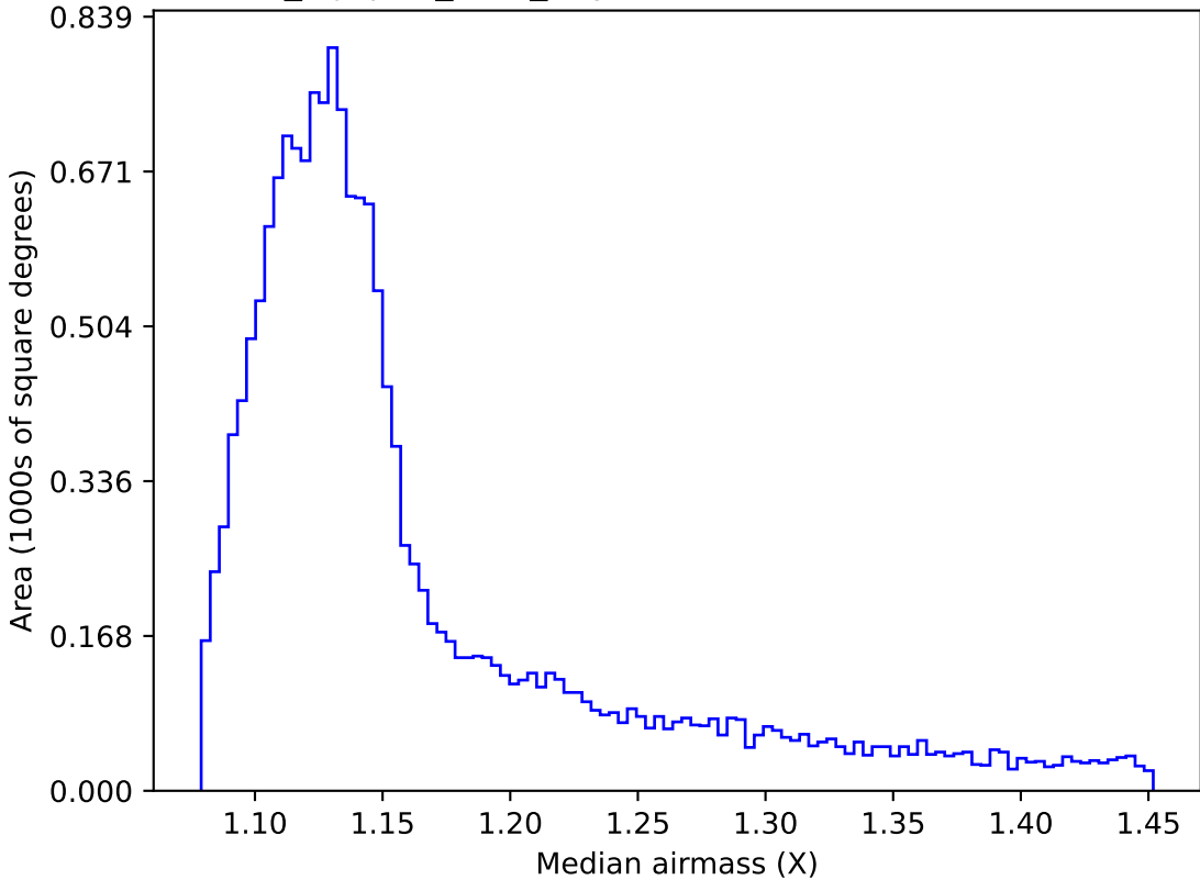
noroll_mjdp60_v3.4_10yrs WFD z band: Median airmass
