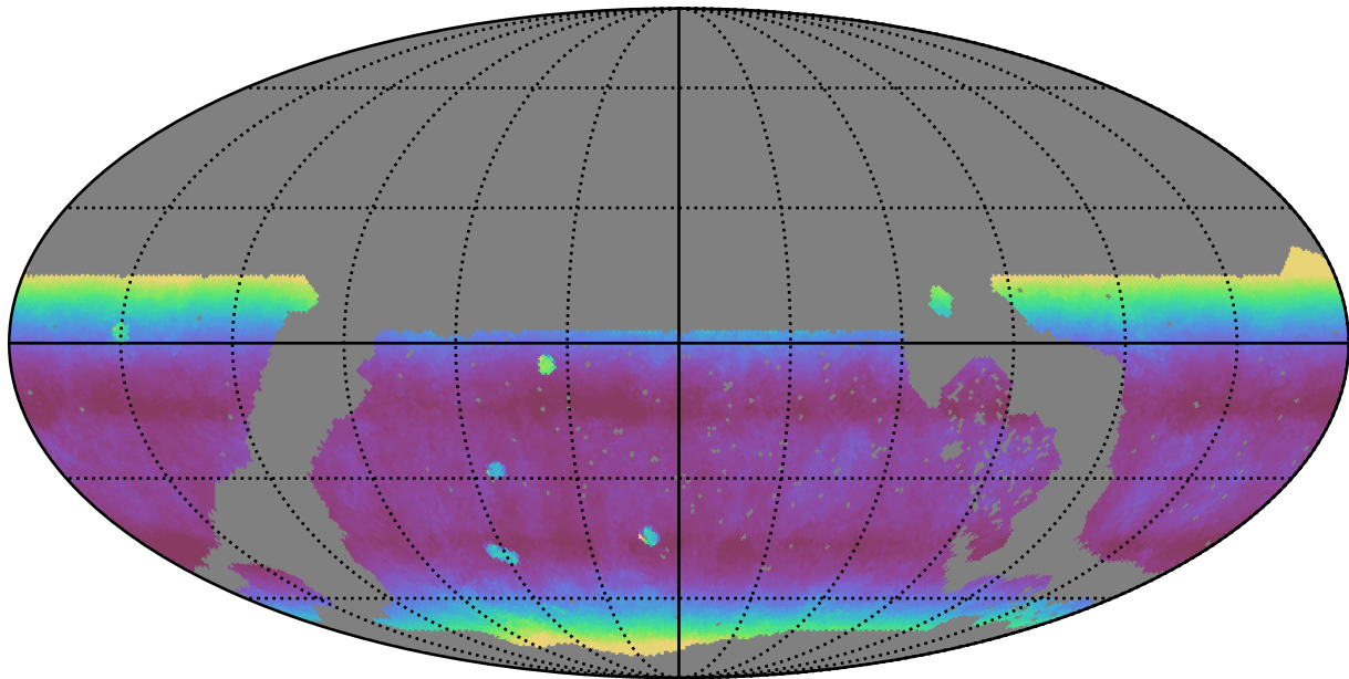
noroll_mjdp60_v3.4_10yrs WFD y band: Median airmass
