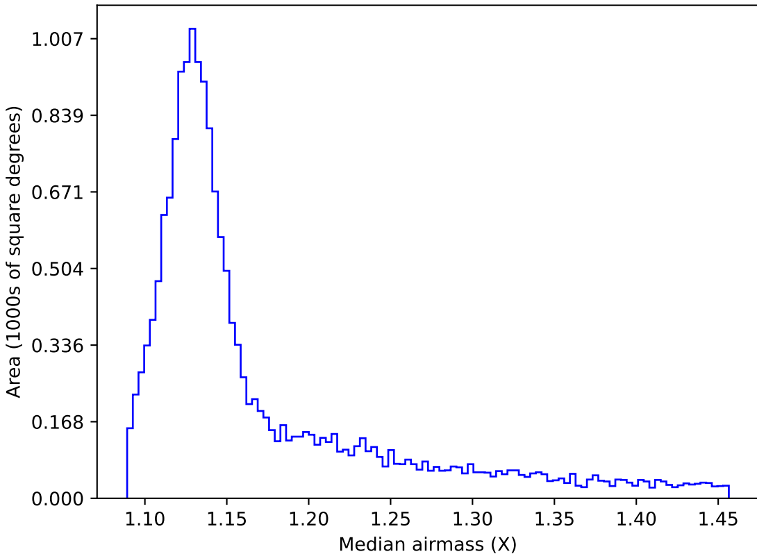
noroll_mjdp60_v3.4_10yrs WFD y band: Median airmass
