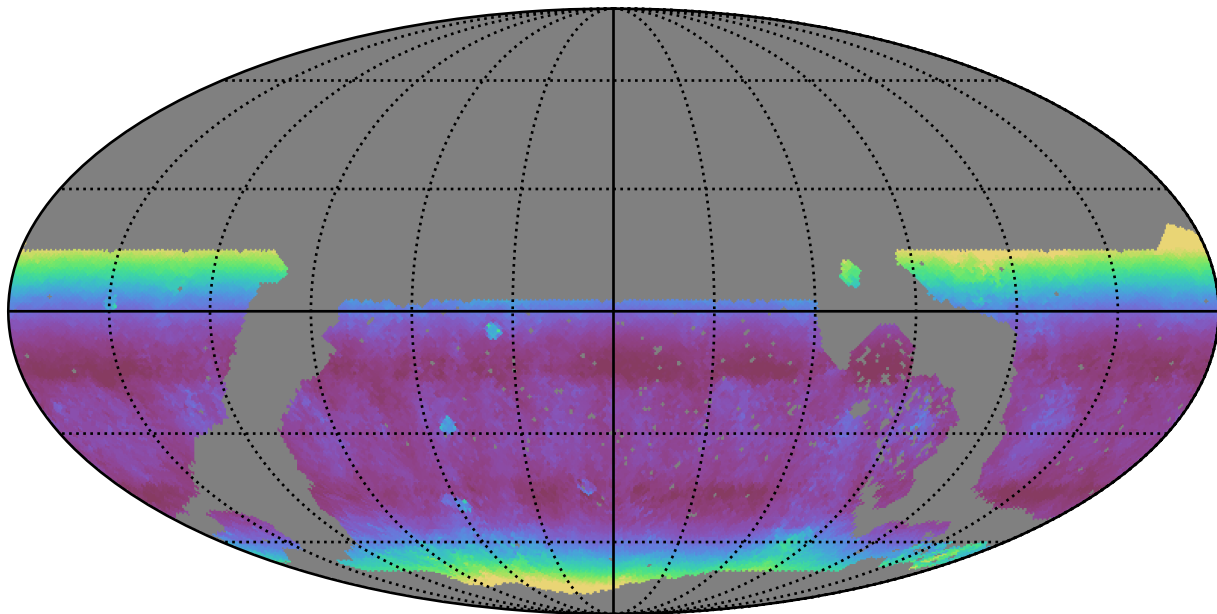
noroll_mjdp60_v3.4_10yrs WFD u band: Median airmass
