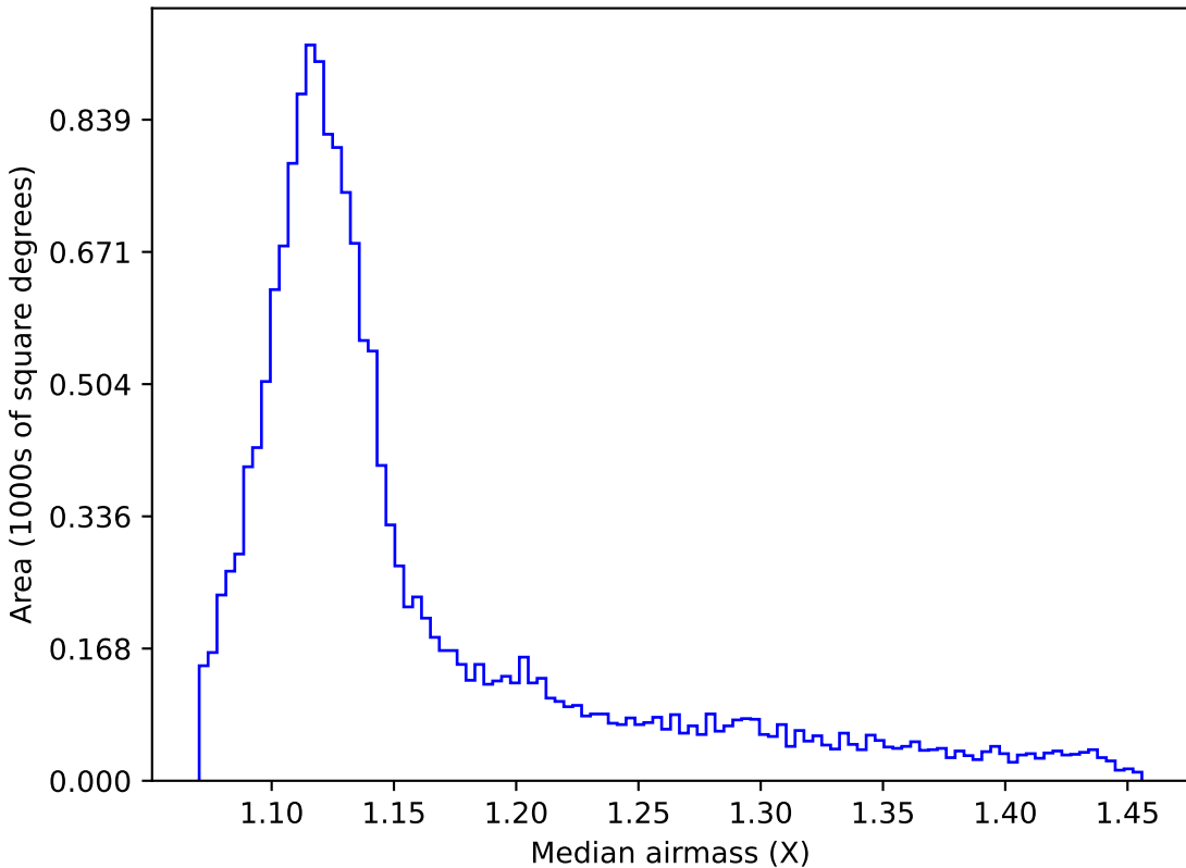
noroll_mjdp60_v3.4_10yrs WFD u band: Median airmass
