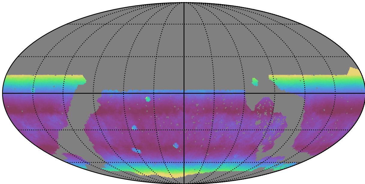
noroll_mjdp60_v3.4_10yrs WFD r band: Median airmass
