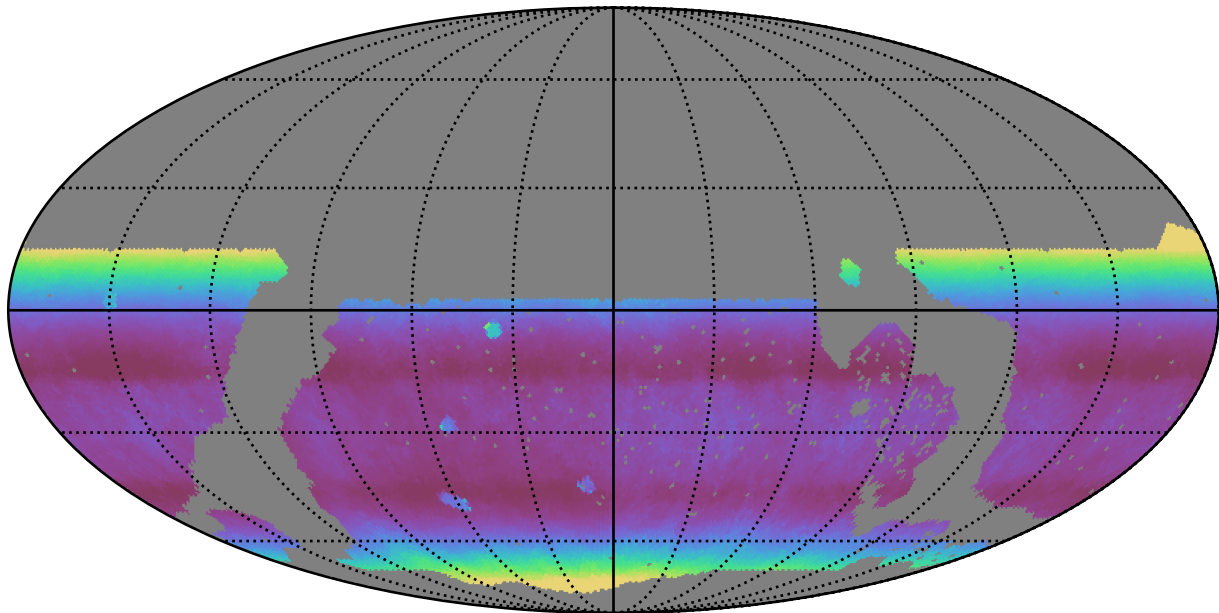
noroll_mjdp60_v3.4_10yrs WFD i band: Median airmass
