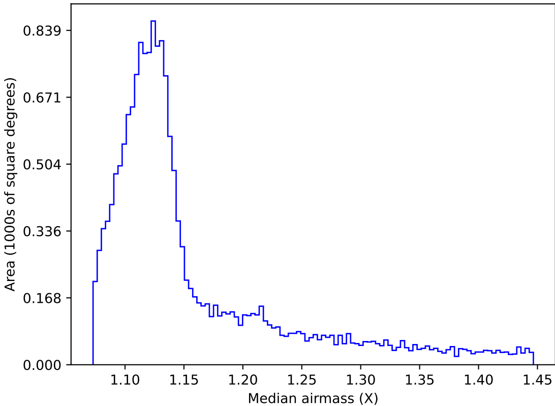
noroll_mjdp60_v3.4_10yrs WFD i band: Median airmass
