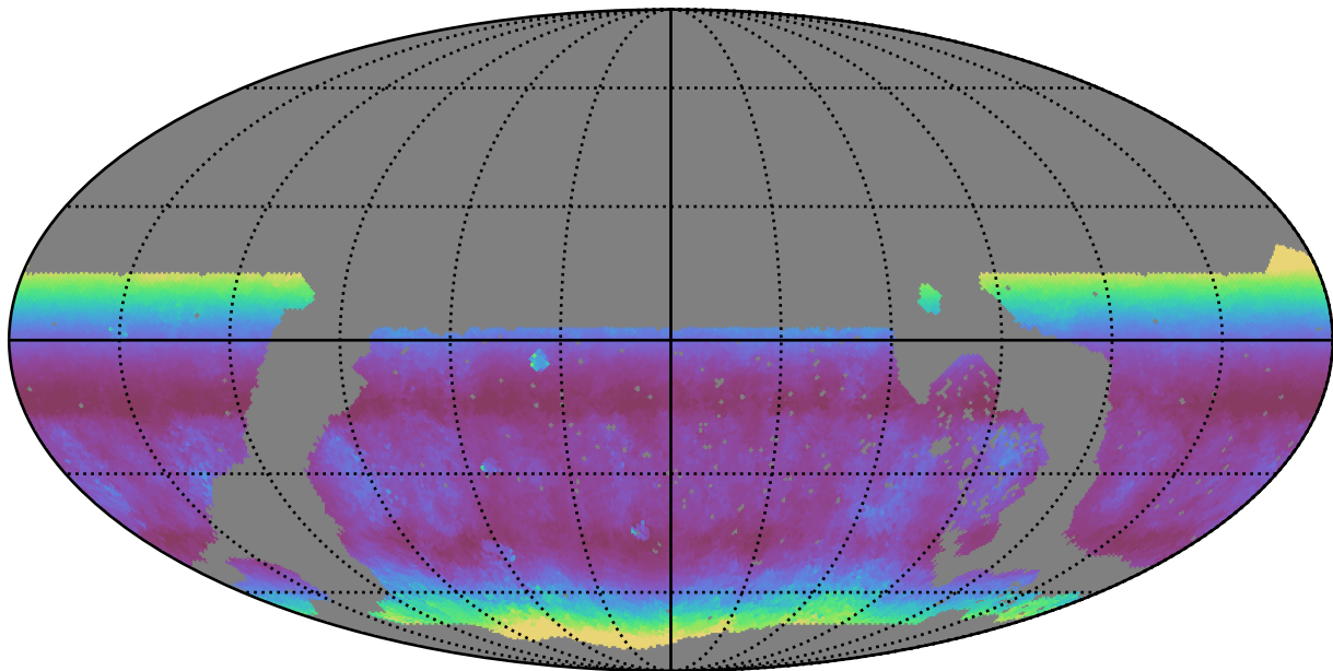
noroll_mjdp60_v3.4_10yrs WFD g band: Median airmass
