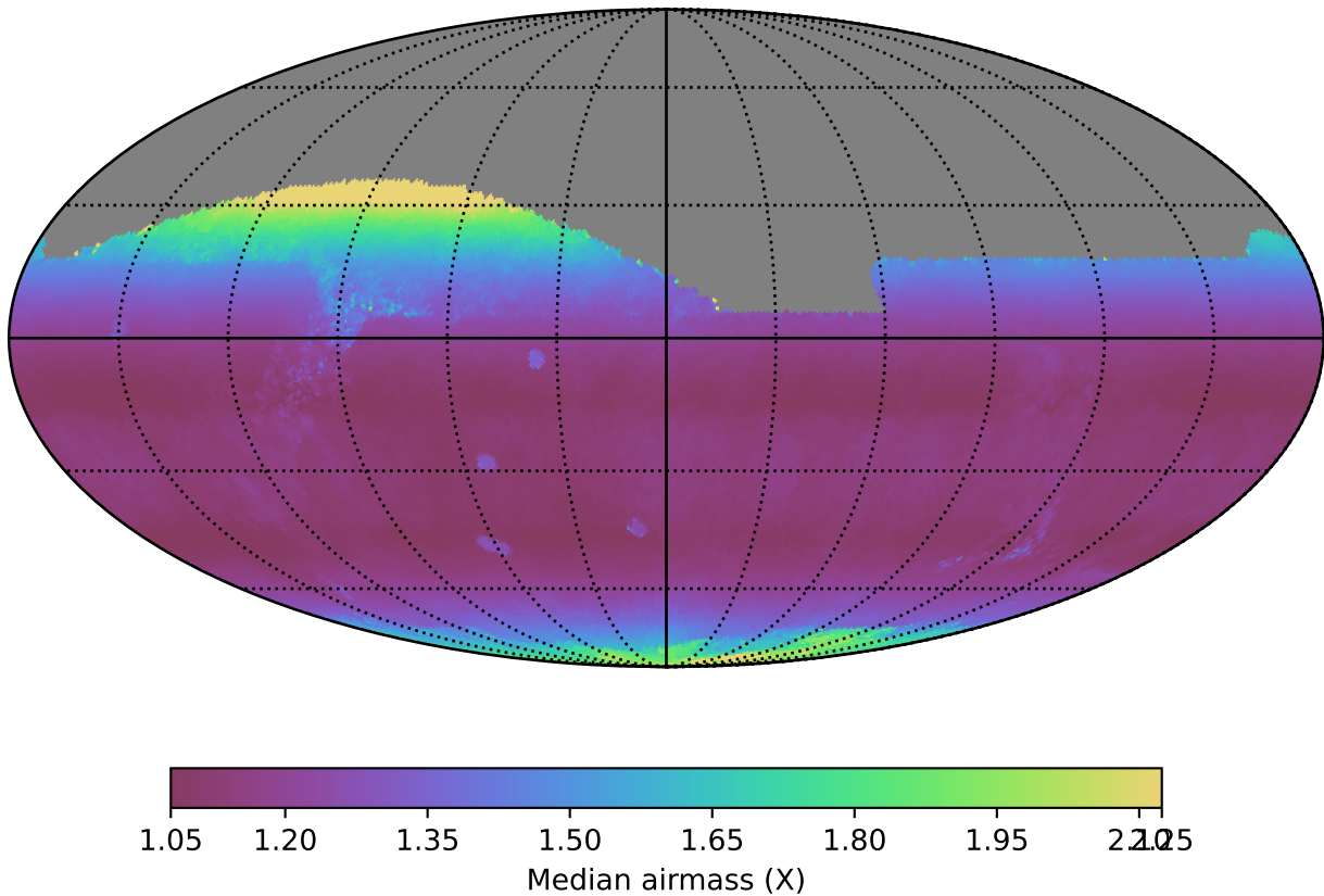
noroll_mjdp60_v3.4_10yrs All sky z band: Median airmass
