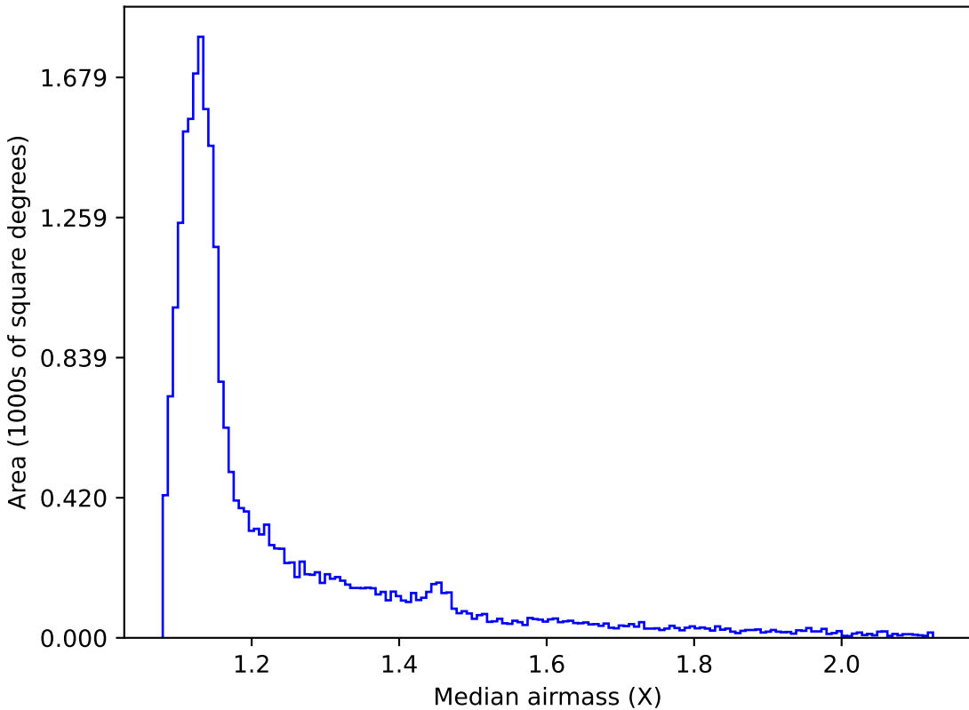
noroll_mjdp60_v3.4_10yrs All sky z band: Median airmass
