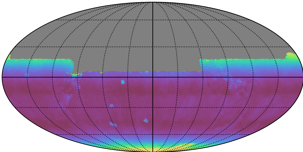
noroll_mjdp60_v3.4_10yrs All sky y band: Median airmass
