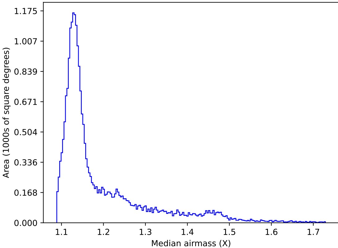
noroll_mjdp60_v3.4_10yrs All sky y band: Median airmass
