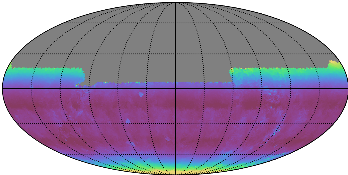
noroll_mjdp60_v3.4_10yrs All sky u band: Median airmass
