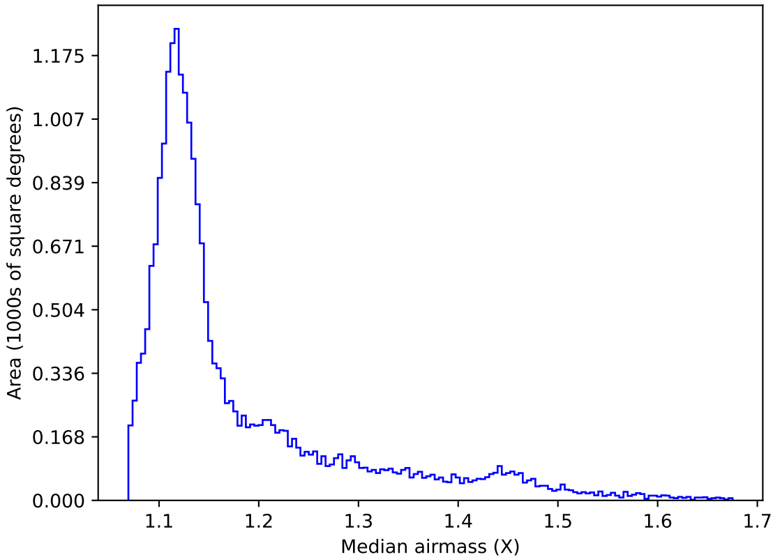
noroll_mjdp60_v3.4_10yrs All sky u band: Median airmass
