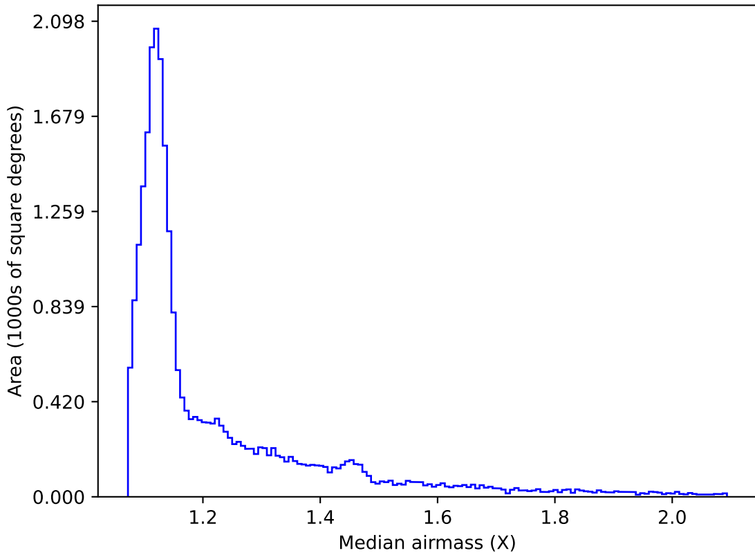
noroll_mjdp60_v3.4_10yrs All sky r band: Median airmass
