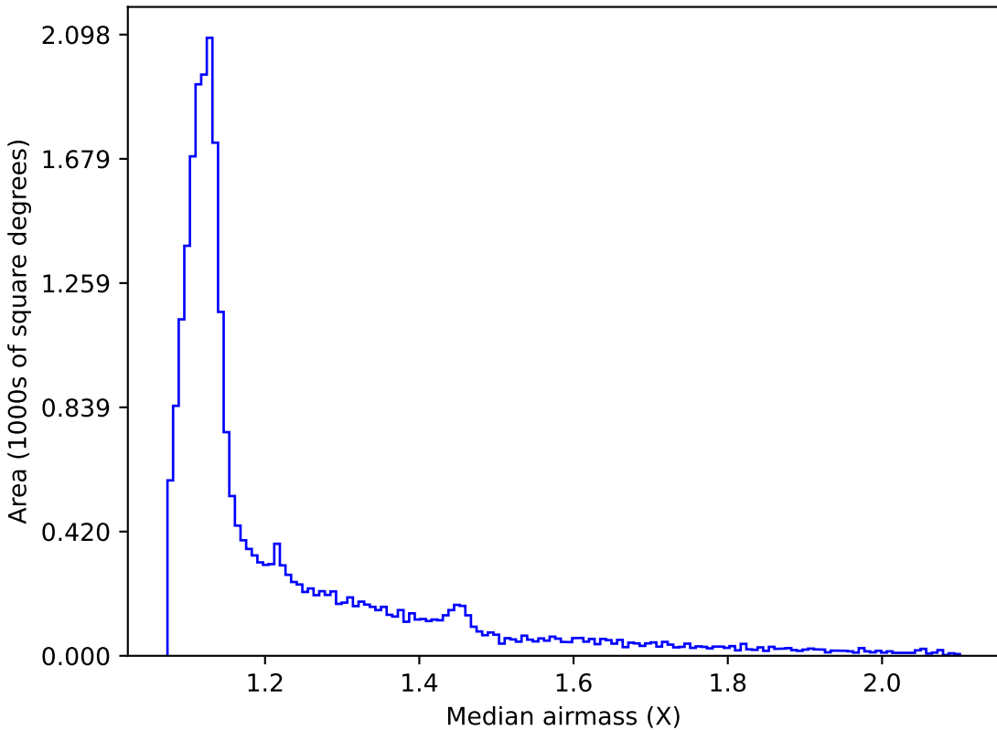
noroll_mjdp60_v3.4_10yrs All sky i band: Median airmass
