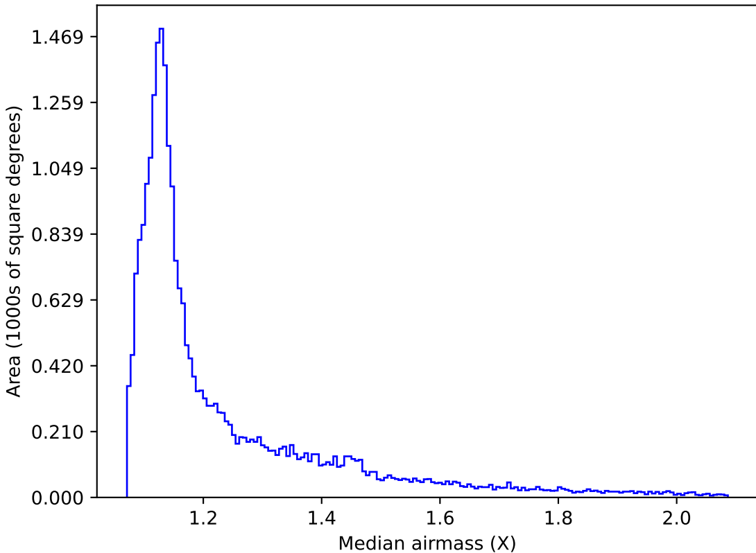
noroll_mjdp60_v3.4_10yrs All sky g band: Median airmass
