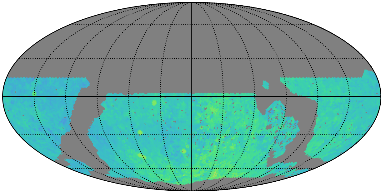
noroll_mjdp60_v3.4_10yrs WFD z band: Median Season Length
