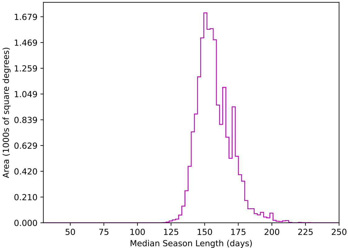
noroll_mjdp60_v3.4_10yrs WFD z band: Median Season Length
