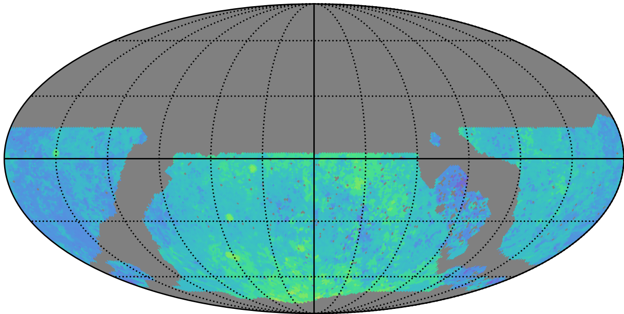
noroll_mjdp60_v3.4_10yrs WFD y band: Median Season Length
