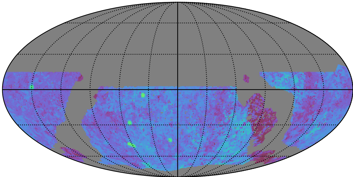
noroll_mjdp60_v3.4_10yrs WFD u band: Median Season Length
