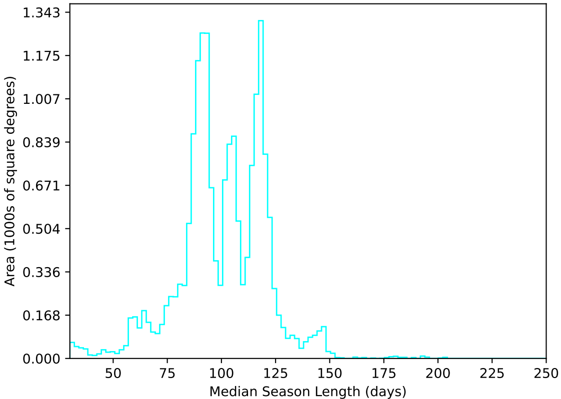
noroll_mjdp60_v3.4_10yrs WFD u band: Median Season Length
