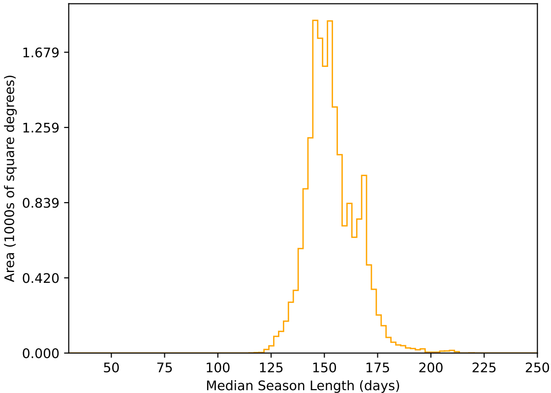
noroll_mjdp60_v3.4_10yrs WFD r band: Median Season Length
