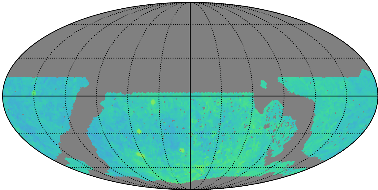
noroll_mjdp60_v3.4_10yrs WFD i band: Median Season Length
