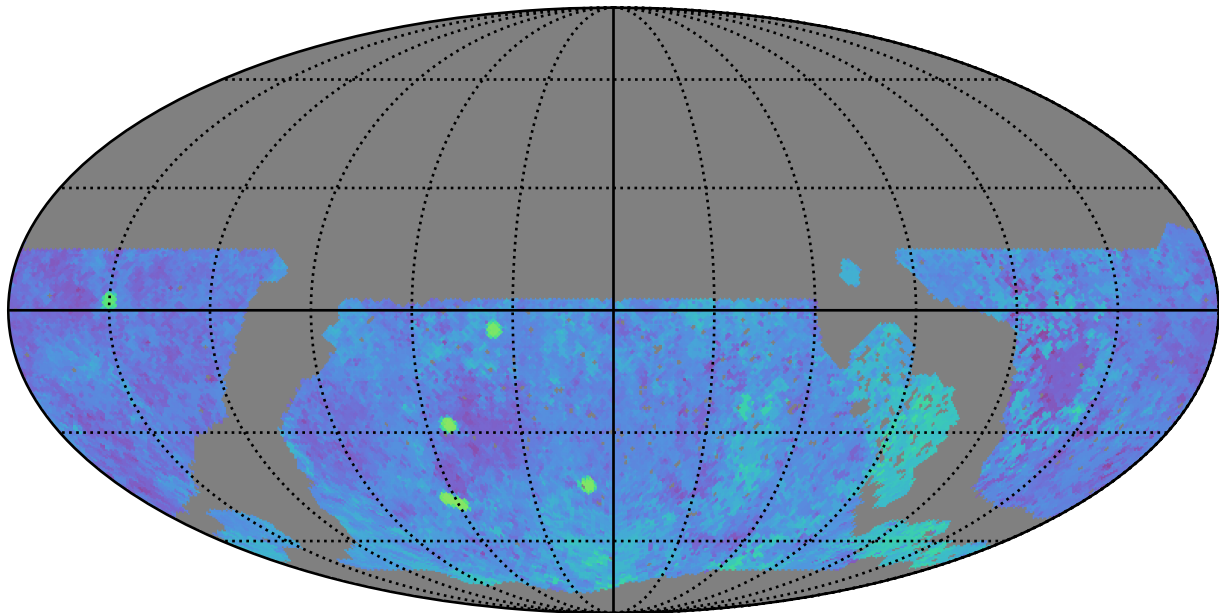
noroll_mjdp60_v3.4_10yrs WFD g band: Median Season Length
