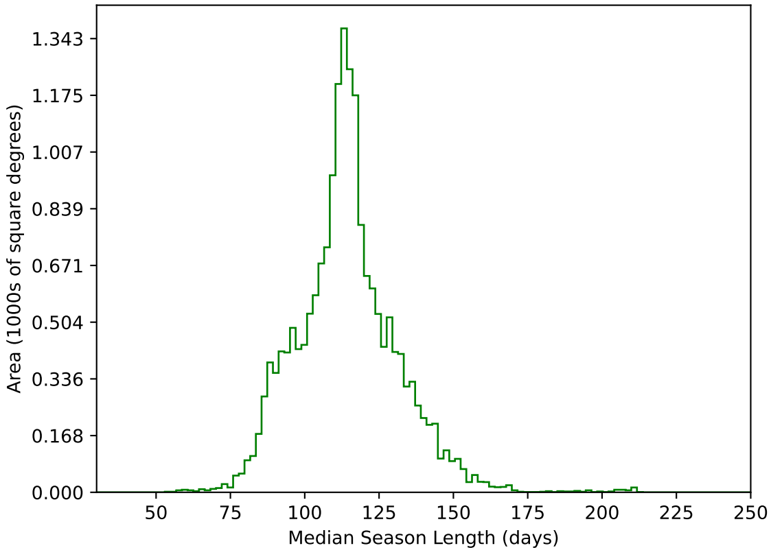
noroll_mjdp60_v3.4_10yrs WFD g band: Median Season Length
