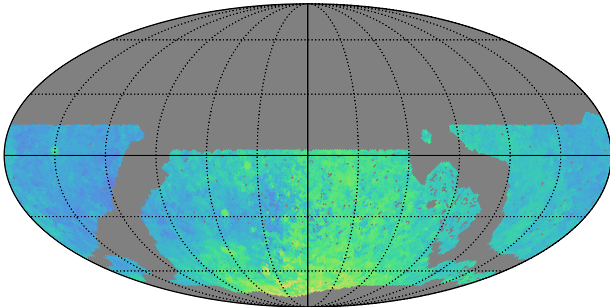
noroll_mjdp60_v3.4_10yrs WFD all bands: Median Season Length
