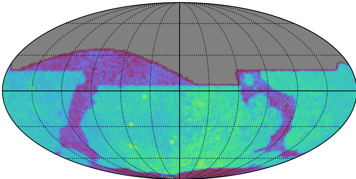
noroll_mjdp60_v3.4_10yrs All sky z band: Median Season Length
