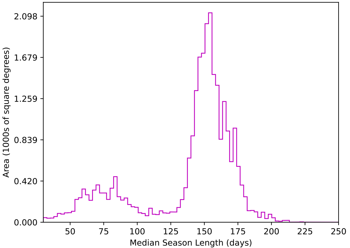
noroll_mjdp60_v3.4_10yrs All sky z band: Median Season Length
