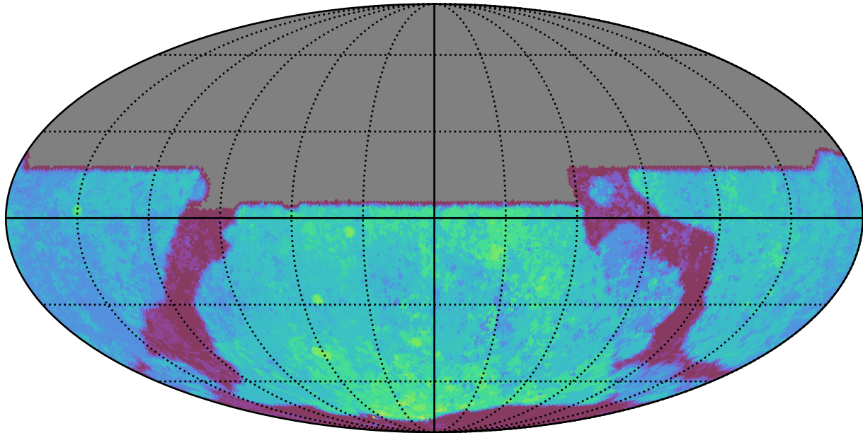
noroll_mjdp60_v3.4_10yrs All sky y band: Median Season Length
