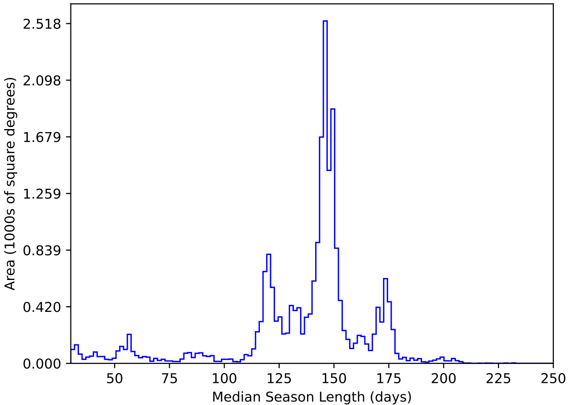
noroll_mjdp60_v3.4_10yrs All sky y band: Median Season Length
