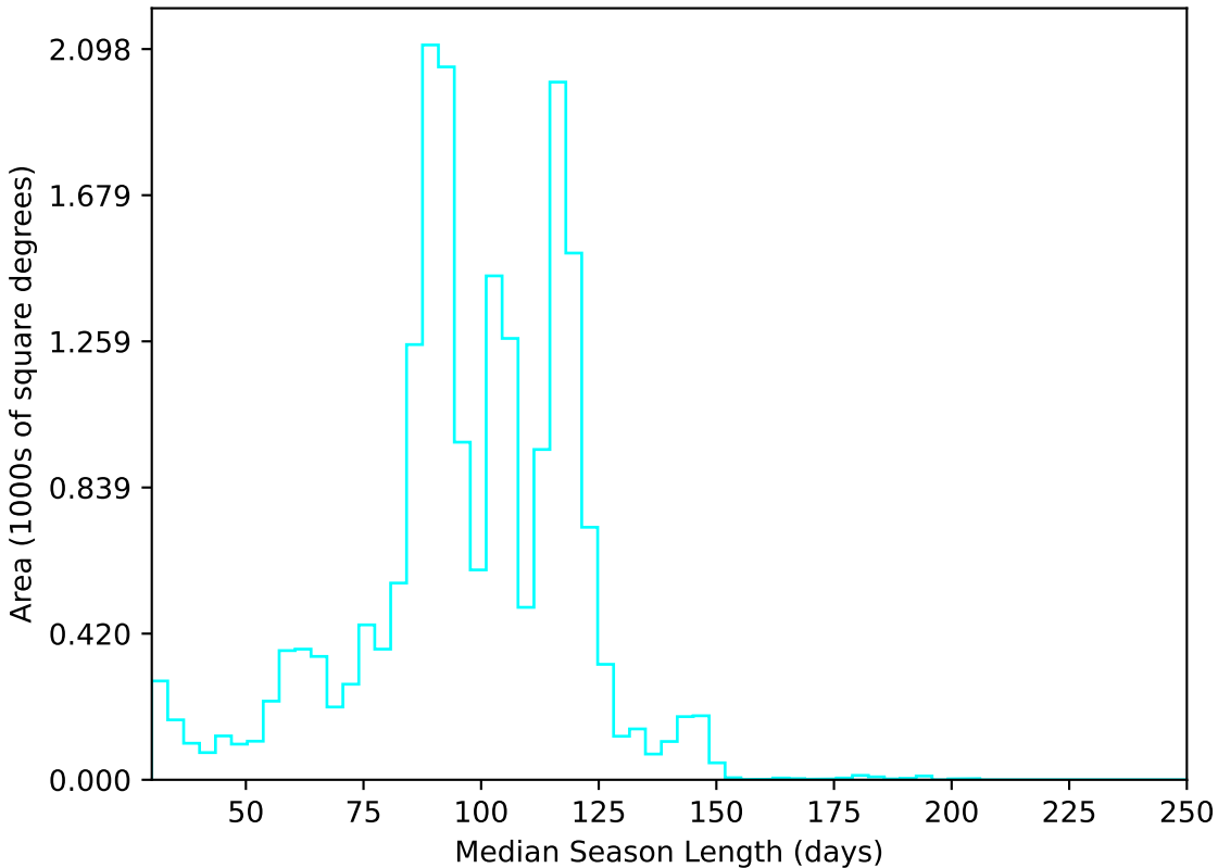
noroll_mjdp60_v3.4_10yrs All sky u band: Median Season Length
