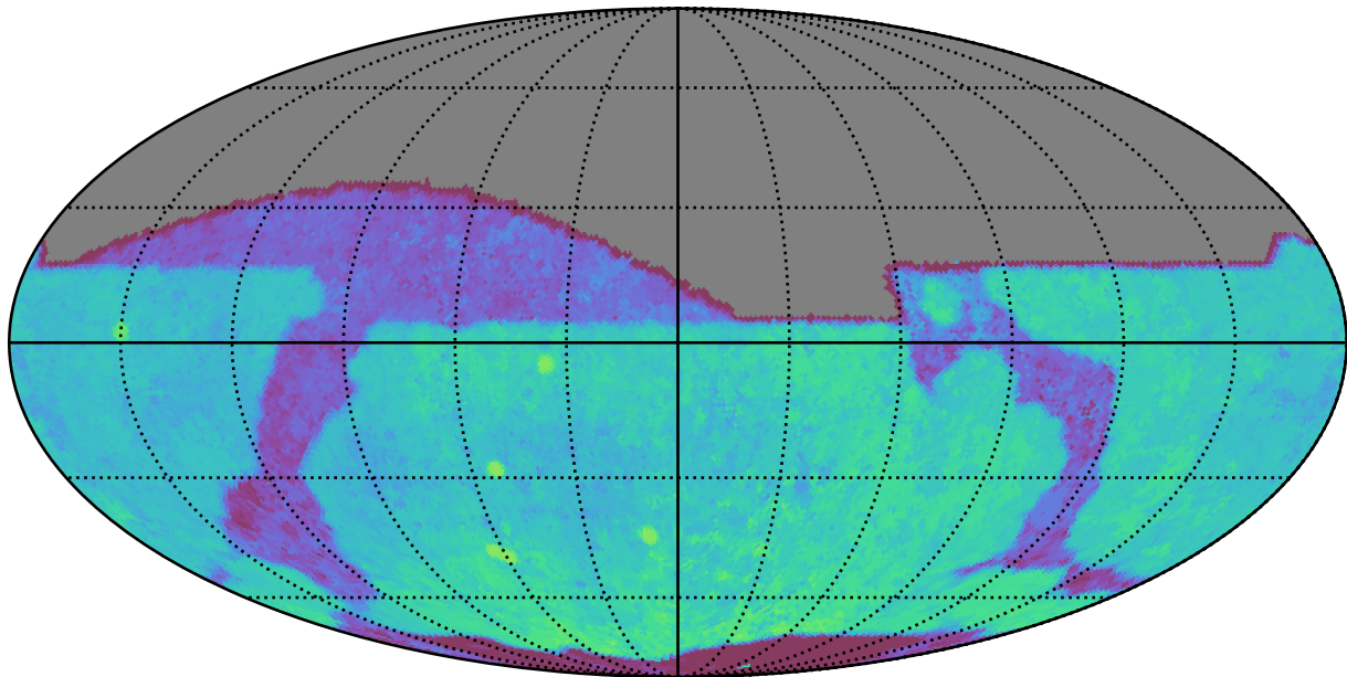
noroll_mjdp60_v3.4_10yrs All sky r band: Median Season Length
